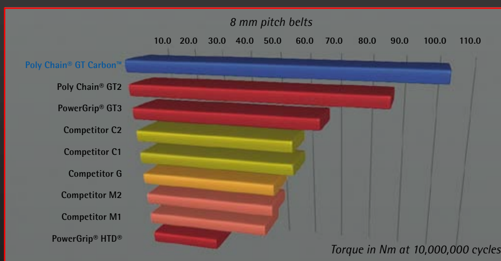
Poly Chain® GT Carbon™ versus competitors' belts
